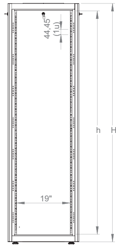
Dimensions in width and height
